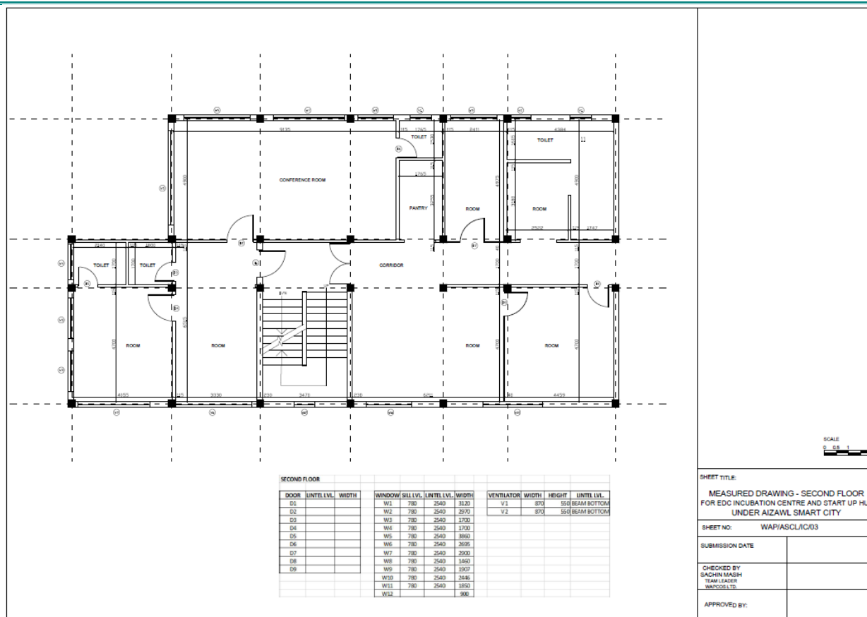
FIGURE 1-10: SECOND FLOOR PLAN
