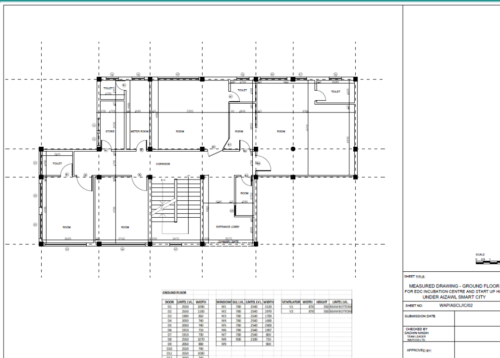
FIGURE 1-9: GROUND FLOOR PLAN
